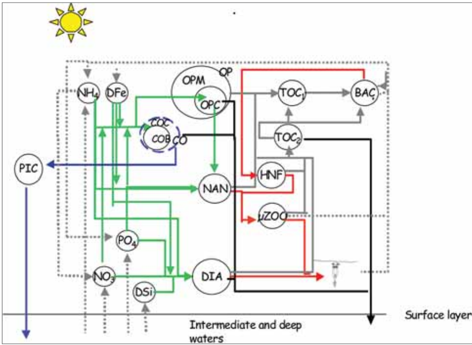
Figure 3.14. Structure of the ecosystem model SWAMCO-4, including processes (arrows) and state variables (including major nutrients \text{NH}_4 : ammonium; \text{NO}_3 : nitrate; \text{PO}_4 : phosphate; \text{DSi} : dissolved silica; and dissolved iron \text{DFe} ). The model explicitly details the dynamics of 4 relevant phytoplankton groups: i) DIA: diatoms; ii) NAN: pico/nano phytoflagellate; iii) OP, OPC, OPM: Phaeocystis colony, cell, colony polysaccharide matrix; iv) CO, COB, COC: coccolithophorid cell, biomass, attached coccoliths and PIC: COC+detached coccoliths. \text{TOC}_i : fast ( i=1 ) and slowly ( i=2 ) biodegradable organic matter; BAC: bacteria; HNF: heterotrophic nanoflagellate; \mu\text{ZOO} : microzooplankton. The model integrates knowledge on mechanisms controlling biological productivity and the structure of the planktonic ecosystem. (Source: Pasquer et al. 2005) 51
