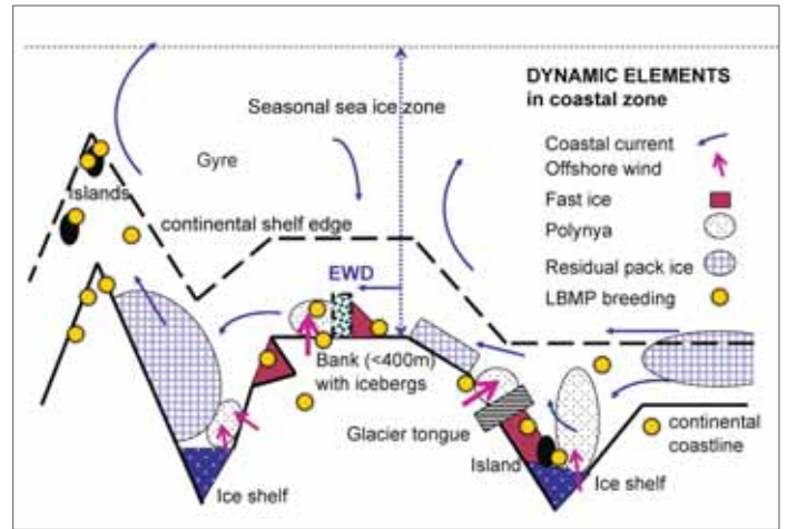
Figure 2.16. Conceptual schematic diagram of the Antarctic coastal marine zone highlighting processes that may drive, or are involved in, (bio) regionalisation. Basic elements are the coastline, the continental shelf edge, and islands. Other fixed features are also labelled. Residual pack ice in this case refers to regions of perennial sea ice i.e., sea ice that persists through the summer to survive the melt season. Fast ice and polynyas etc. are more extensive in reality than depicted here. Figure developed by H. Keys (DOC, New Zealand) and R. Massom, based on other work including Beaman and Harris (2005) 2 and Massom et al. (2001) 16 .
