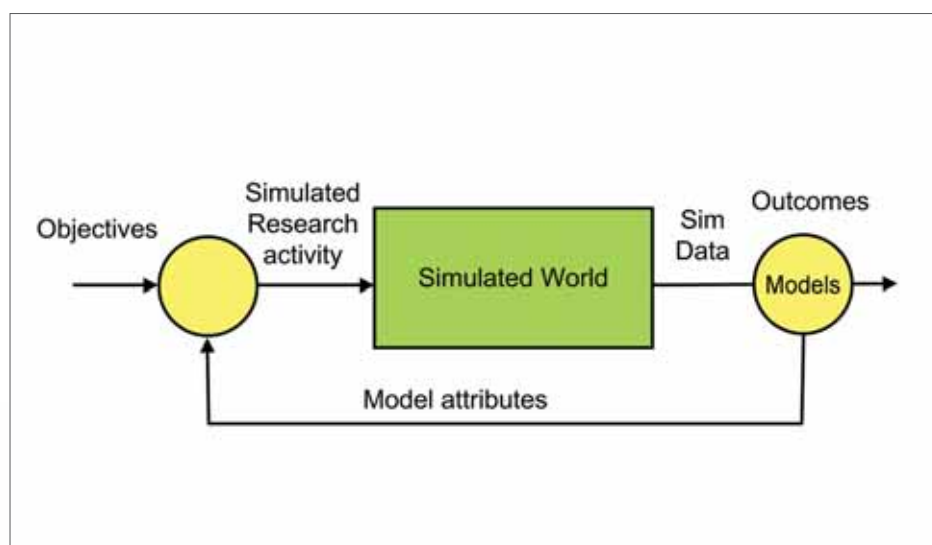
Figure 6.1. Schematic of a simulation for evaluating a monitoring and assessment strategy using the Management Oriented Paradigm.
