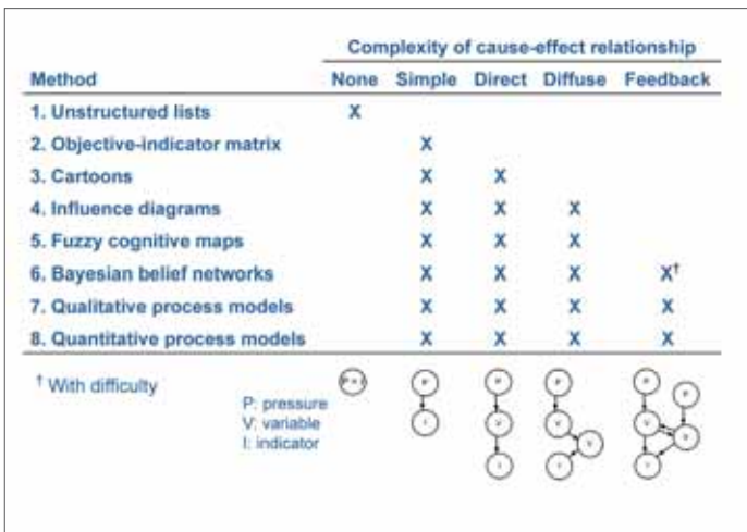
Figure 5.5. Sufficient methodologies for identifying ecological indicators (Hayes et al. 2008) 17 . Pressure is the external pressure applied to the system, such as climate change. A variable is a component of the system. The indicator is what is measured.
