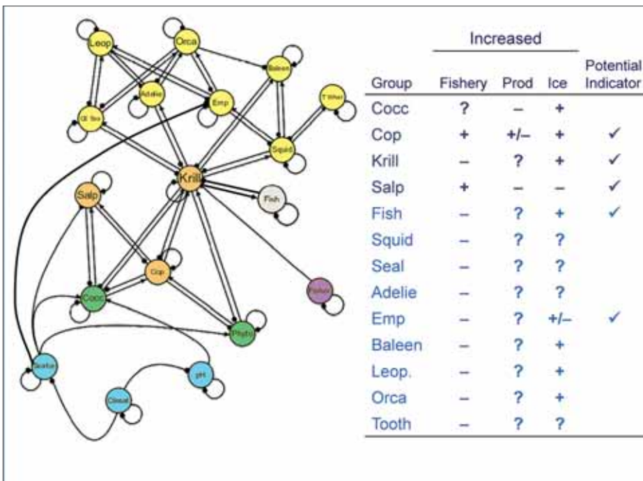
Figure 5.6. Qualitative model of a 'krill-based food web' (following de la Mare & Dambacher, unpublished). The network shows interactions amongst components of this illustrative ecosystem: sea ice, climate, pH = acidity, Cocc = Coccolithophorids, Phyto = Phytoplankton, Cop = Copepods, Salps, Krill, Fish, Squid, CE Seal = Crabeater seals, Adelie penguins, Emp = emperor penguins, Leop = Leopard seals, Orca, Baleen whales, T. Whal = toothed whales. The table shows the results of a qualitative assessment of the impacts of press perturbations on each group following the method of Dambacher et al. (2007, 2009) 7, 8 . Rows correspond to each group from the network plus the responses from individual press perturbations from an increased krill fishery, increased productivity (Prod) and an increase in sea ice. '-' indicates a decline in the group while '+' indicates an increase. '?' indicates a confounded response. Potential indicators are checked on the basis of a clear signal in both fishery and ice as well as a capability to monitor them.
