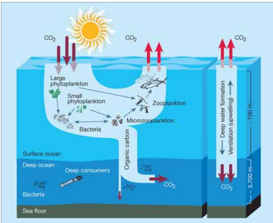
Figure 2.9. The ‘biological pump’ is a collective property of a complex phytoplankton-based food web. Together with the ‘solubility pump’ (right), which is driven by chemical and physical processes, it maintains a sharp gradient of \text{CO}_2 between the atmosphere and the deep oceans. Using sunlight for energy and dissolved inorganic nutrients, phytoplankton convert \text{CO}_2 to organic carbon, which forms the base of the marine food web. As the carbon passes through consumers in surface waters, most of it is converted back to \text{CO}_2 and released to the atmosphere. But some finds its way to the deep ocean where it is remineralized back to \text{CO}_2 by bacteria. The net result is transport of \text{CO}_2 from the atmosphere to the deep ocean, where it stays, on average, for roughly 1,000 years. The food web’s structure and the relative abundance of species influences how much \text{CO}_2 will be pumped to the deep ocean. This structure is dictated largely by the availability of inorganic nutrients such as nitrogen, phosphorus, silicon and iron. Iron is the main limiting nutrient in the Southern Ocean. (Reprinted by permission from Macmillan Publishers Ltd: Nature (Chisholm 2000), copyright 2000, http://www.nature.com/index.html )
