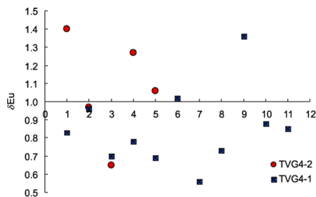
Figure 8 Varying patterns of \delta\text{Eu} from TVG4-1 and TVG4-2.
