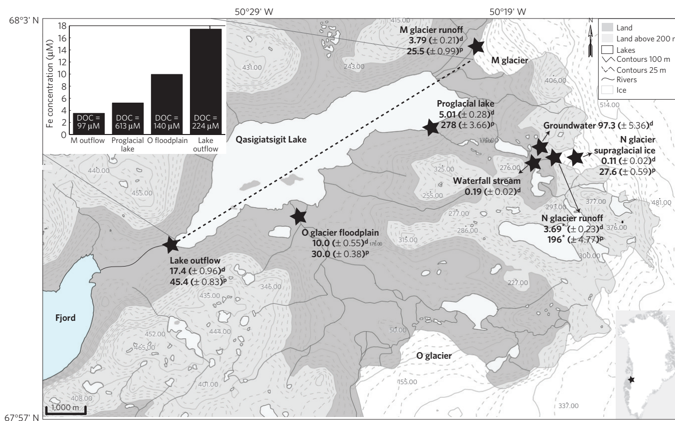
Figure 1 | Map of primary sample locations on the southwestern margin of the GrIS (1:100, adapted from NunaGIS). Approximate sample locations (black stars) are named in italicized text, and contour elevations are shown in metres. Average dissolved (d; <0.2 μm) and particulate (oxyhydr)oxide (p; >0.7 μm) Fe concentrations and errors (±) in measurements are reported in micromolar concentrations. The N glacier runoff values (*) are discharge-weighted average concentrations. The dFe concentrations in samples along a transect (black dashed line) are plotted in the inset, with the DOC concentrations (previously reported in ref. 19) measured in each sample also shown.
