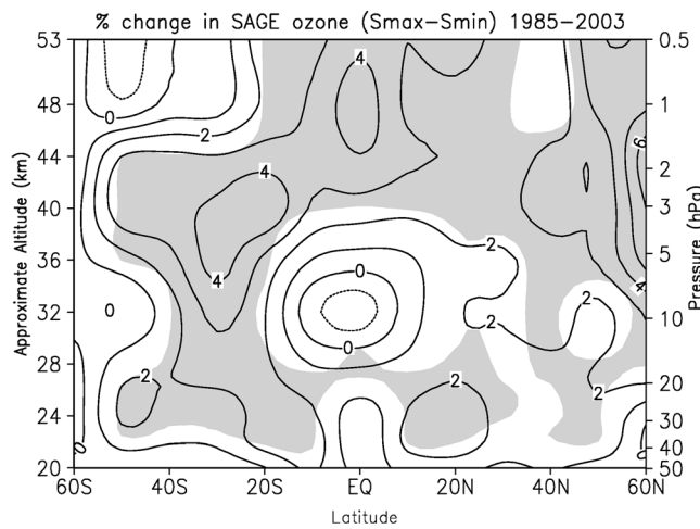
Figure 10. Annual averaged estimate of S_{max} minus S_{min} ozone differences (%) from a multiple regression analysis of SAGE II ozone data for the 1985–2003 period. Shaded areas are significant at the 5% level [from Soukharev and Hood, 2006].
