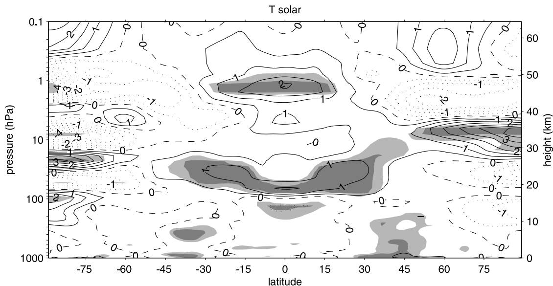
Figure 11. Annual averaged estimate of S_{max} minus S_{min} temperature difference (K) derived from a multiple regression analysis of the European Centre for Medium Range Weather Forecasts (ECMWF) Reanalysis (ERA-40) data set (adapted from Frame and Gray [2010]). Dark and light shaded areas denote statistical significance at the 1% and 5% levels, respectively.
