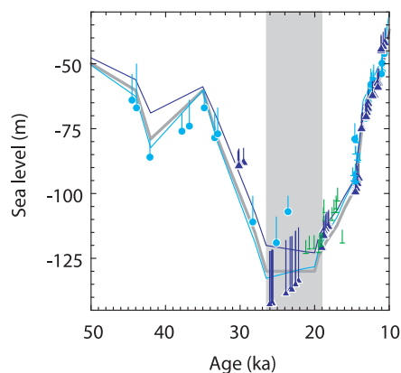
Fig. 2. Sea-level predictions for New Guinea (blue line) and Barbados (purple line) compared to RSL data with depth uncertainty for the interval from 10 to 50 ka from New Guinea (blue circles) (4, 52, 53), Barbados (purple triangles) (5, 54), the Bonaparte Gulf (green half-pluses representing age and depth uncertainty) (8), and the Sunda Shelf (blue half-pluses) (55). Eustatic sea-level time series are shown as a gray line. The vertical gray bar indicates the time of the LGM as defined from the RSL data.
