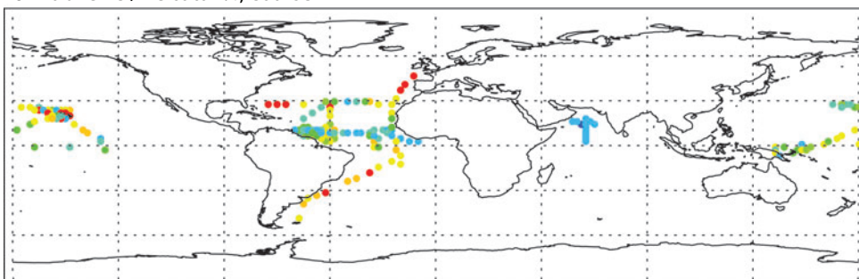
a Labile Fe / Fe total %, coarse
