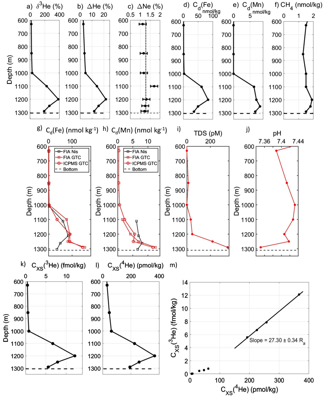
Fig. 3. Loihi profiles of a) , helium isotope ratio anomaly \delta^3\text{He} in %, b) , dissolved helium saturation anomaly in %, c) , dissolved neon saturation anomaly in %, d) , dissolved Fe in nmol kg -1 , e) , dissolved Mn in nmol kg -1 , f) , dissolved CH 4 in nmol kg -1 , g) dissolved Fe (ICPMS for GTC hydrocast only, and FIA for both), h) , dissolved Mn (same as Fe), i) , TDS (pM) from the GTC cast, j) , pH from the GTC cast k) , excess {}^3\text{He} in fmol kg -1 , l) , excess {}^4\text{He} in pmol kg -1 , and m) , correlation between excess {}^3\text{He} and {}^4\text{He} . The dashed line represents the bottom depth at the sampling location.
