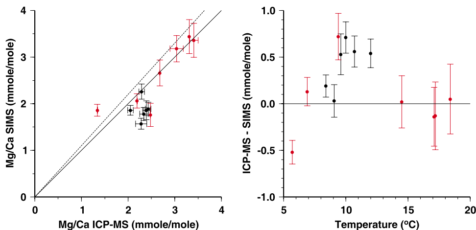
Figure 5. Intercalibration of Mg/Ca ratios based on SIMS measurements and ICP-MS measurements using C. pachyderma samples from the KNR166 multicores. SIMS measurements are the average ( \pm 1 standard error) of all “spots” measured on C. pachyderma tests within the core top. The ICP-MS measurement is based on several whole tests of C. pachyderma following standard analytical techniques [Marchitto et al. , 2007]. Red symbols denote core tops containing bomb radiocarbon. There is good agreement between the methods except for the cores bathed in waters from 9 to 12°C. The reason for this discrepancy is unclear. The dashed line represents the higher (by 10%) Mg/Ca values which might be expected for the SIMS data, which have not been subjected to any chemical cleaning [Yu et al. , 2007]. The large error bars for the SIMS data preclude testing for this possibility.
